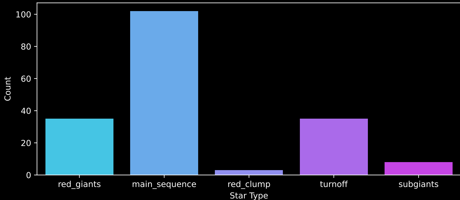
APOGEE DR17 Field: [175+43_MGA] Count plot of Star Type
