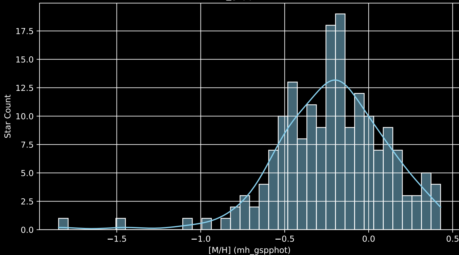
APOGEE DR17 Field: [175+43_MGA [M/H] (mh_gspphot) (n= 180)
