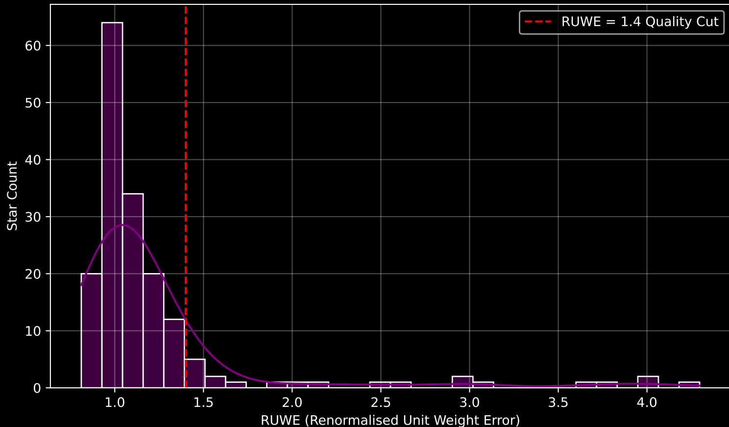
GAPOGEE DR17 Field [175+43_MGA] RUWE Distribution (n= 171)
