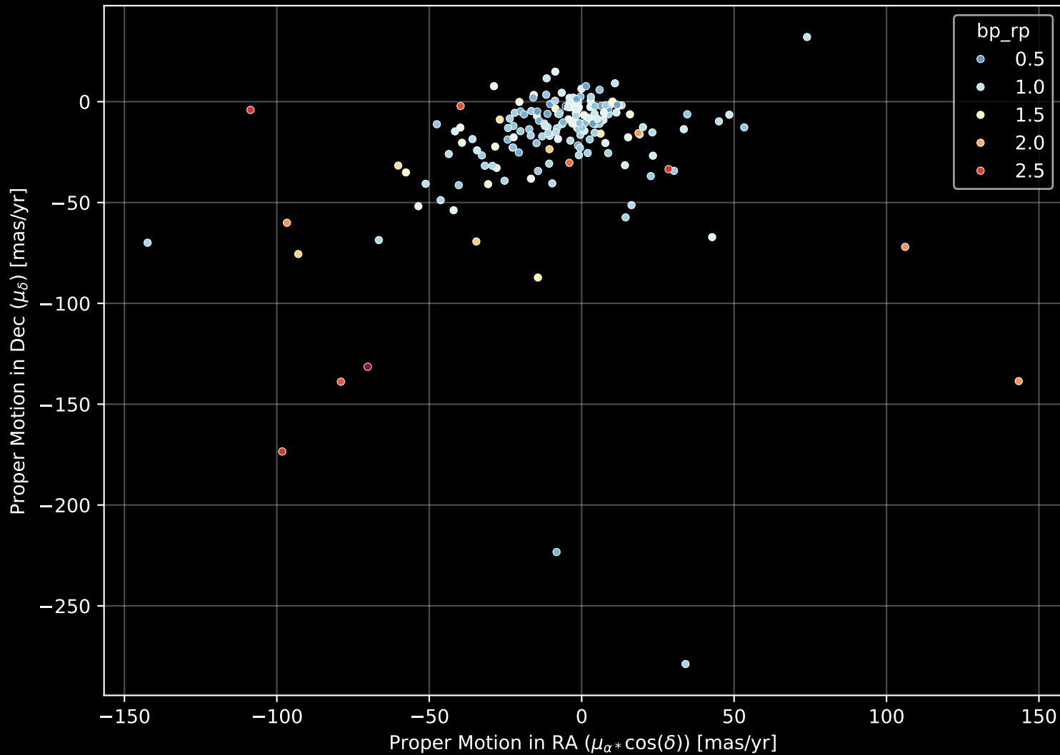
APOGEE DR17 Field: [175+43_MGA] Proper Motion Diagram (n= 183)
