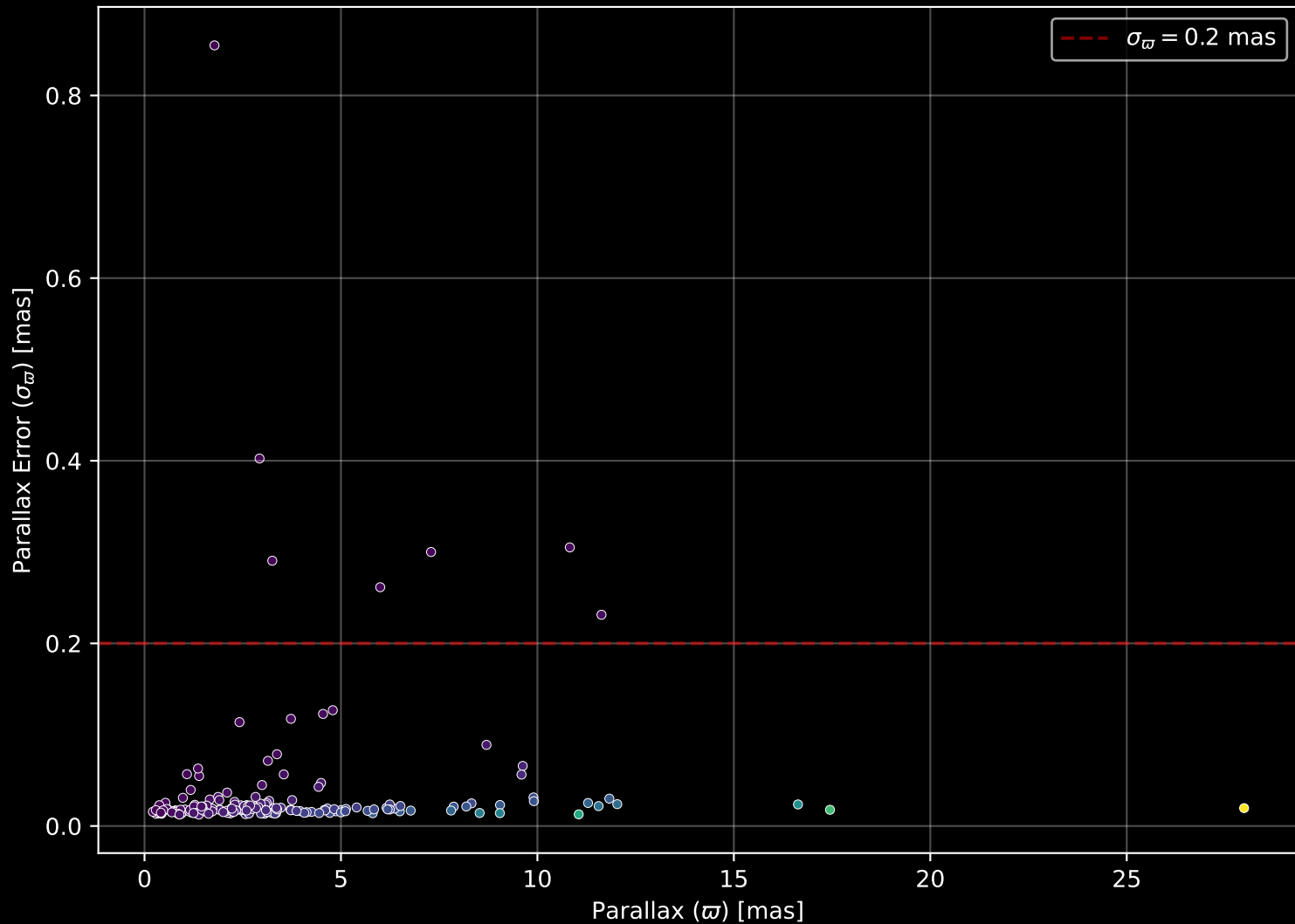
APOGEE DR17 Field: [175+43_MGA] Parallax Quality (n= 183)
