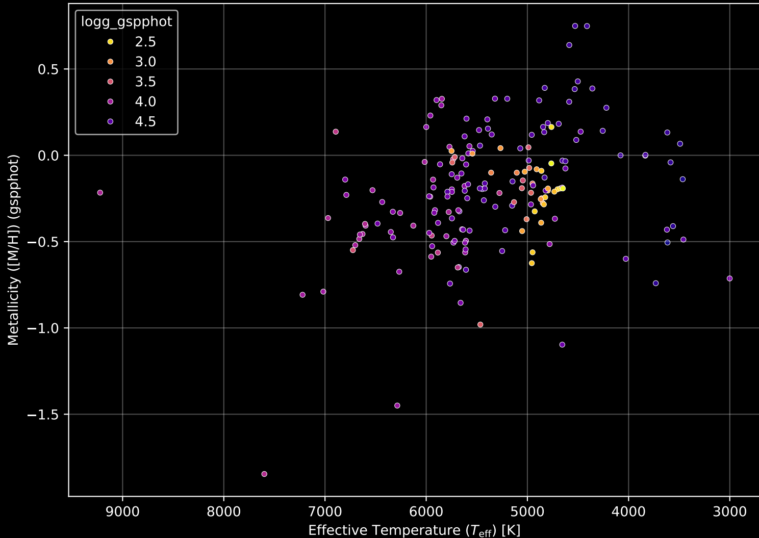
APOGEE DR17 Field: [175+43_MGA] Stellar Population Parameters (n= 183)
